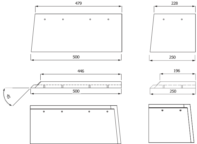
Corner Detail Cutting Guide for L Shape
