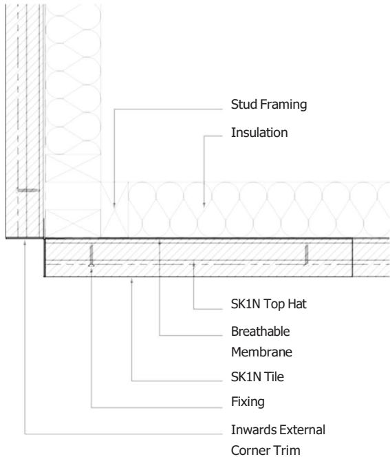
External Corner with Accent Trim
