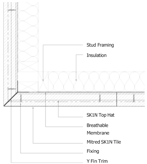
Mitred External Corner with Y Fin Trim
