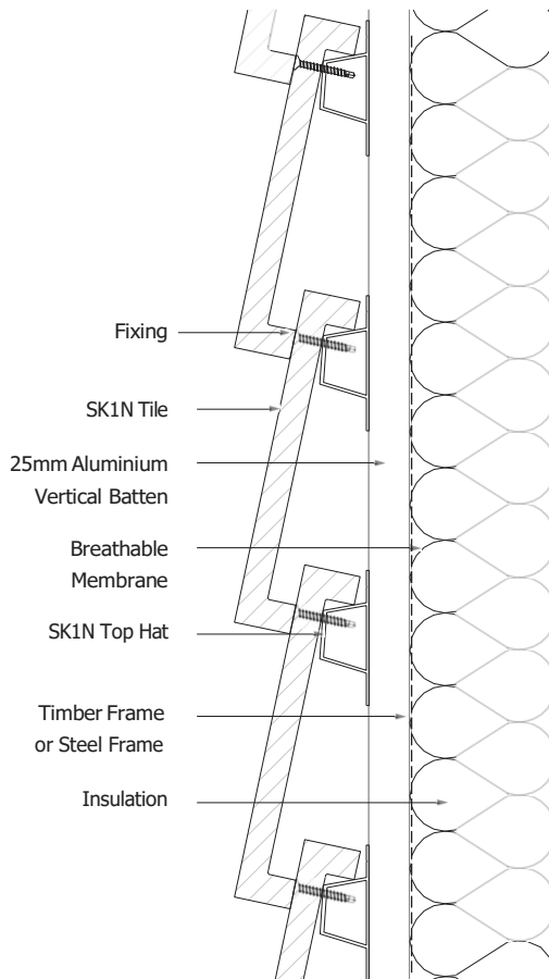
Cavity Fix with SK1N Top Hats
