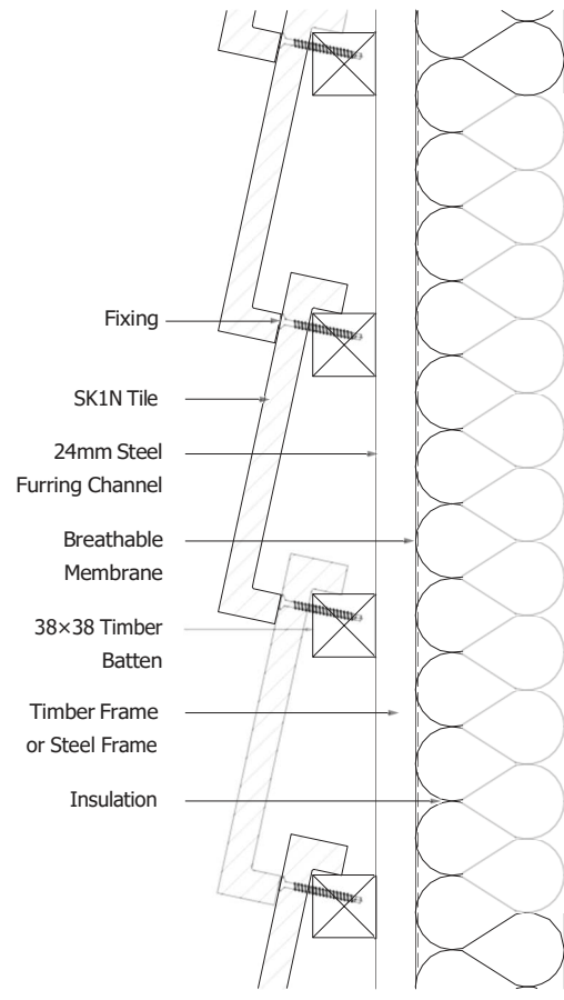
Cavity Fix with Timber Battens
