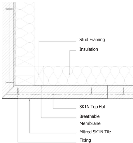
External Corner with Mitre
