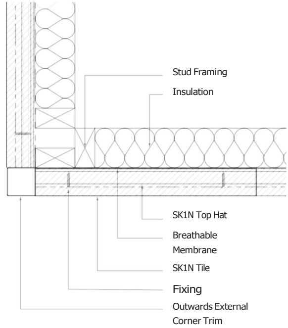
External Corner with Box Trim
